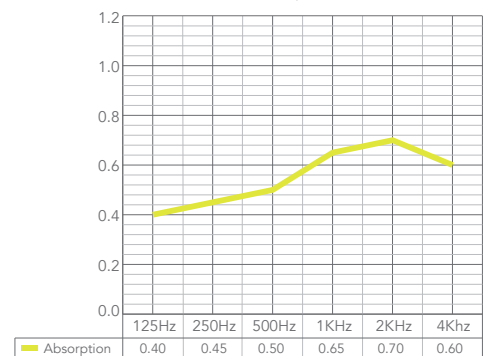
Sound absorption in accordance with ISO 354
