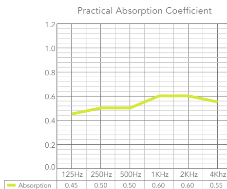
Sound absorption in accordance with ISO 354
