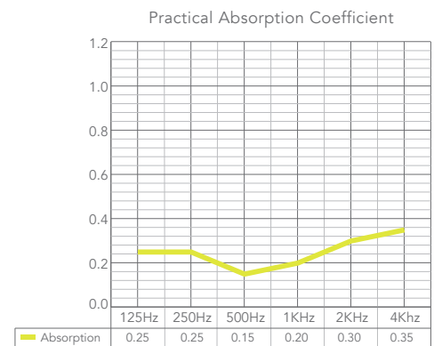
Sound absorption in accordance with ISO 354
