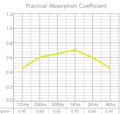
Sound absorption in accordance with ISO 354
